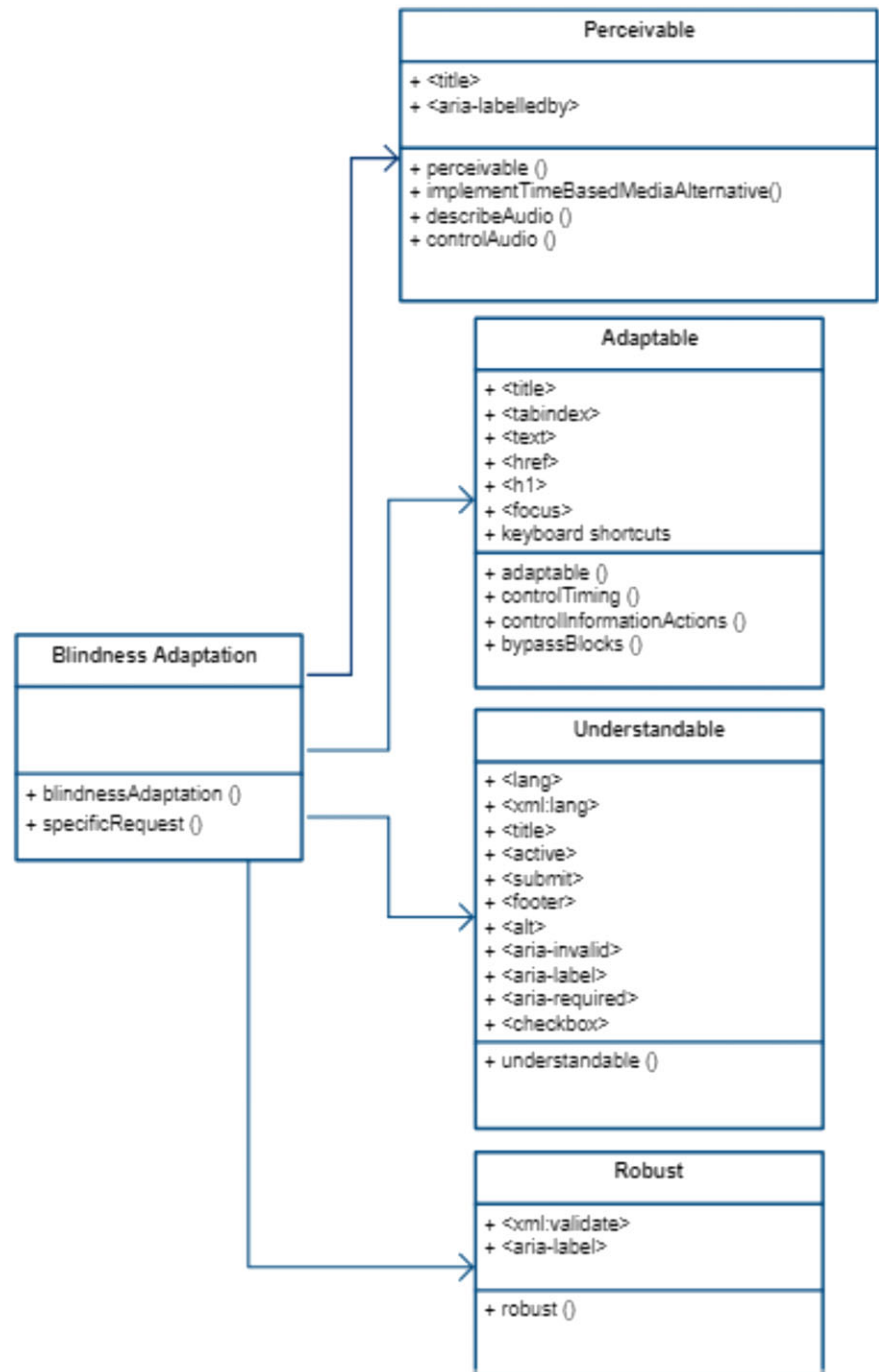
FIGURE 2 Blindness adapter UML class diagram
