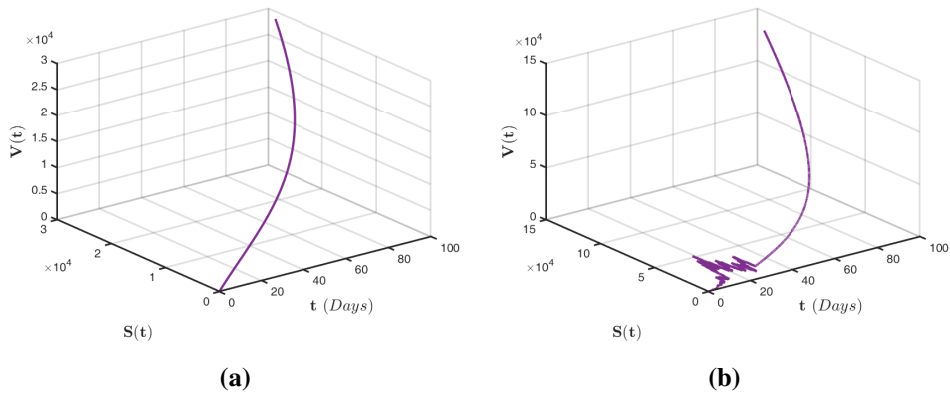
Figure 7. Chaotic behaviour for the model (2.2) and (2.2) for the susceptible individuals s(\xi) and vaccinated v(\xi) when \alpha = 1 with random densities \varphi_1 = \varphi_2 = 0.04 and \varphi_3 = 0.05 .
