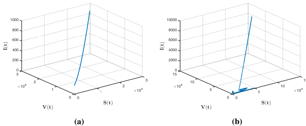
Figure 8. Chaotic behaviour for the model (2.2) and (2.2) for the susceptible individuals s(\xi) , vaccinated v(\xi) and infected individuals i(\xi) when \alpha = 1 with random densities \varphi_1 = \varphi_2 = 0.04 and \varphi_3 = 0.05 .
