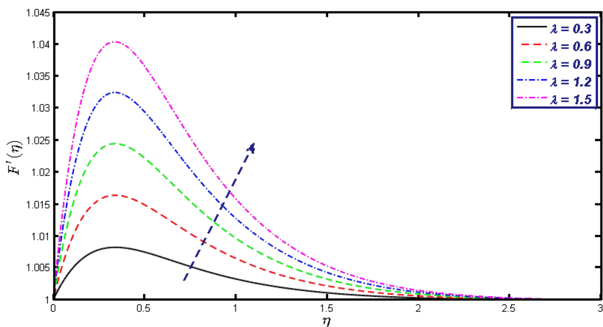
Figure 4. Velocity field for different values of \lambda .
