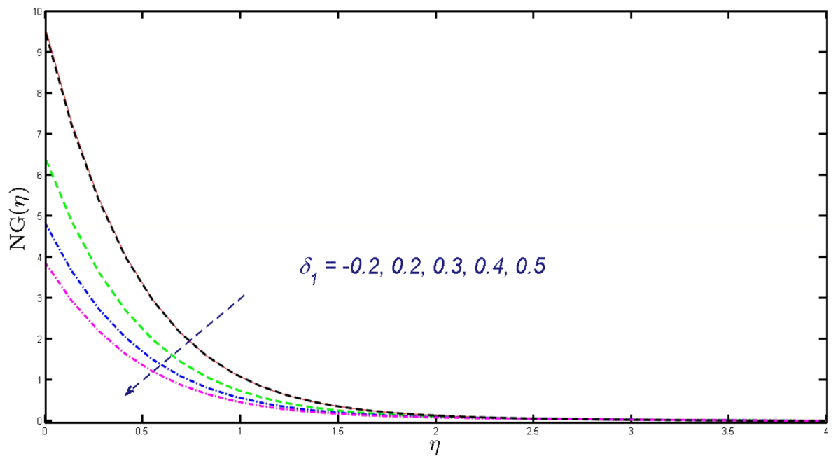
Figure 25. Upshot of NG(\eta) for \delta_1 .
