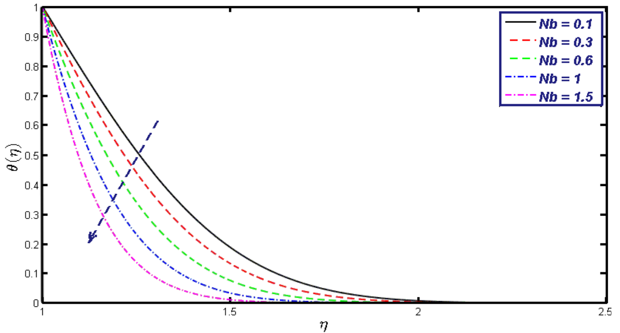
Figure 11. \theta(\eta) field for different values of Nb .
