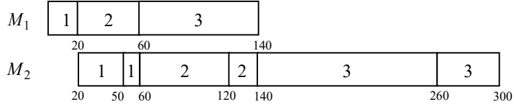
Figure 2. Optimal schedule of the sublots in Example 1
