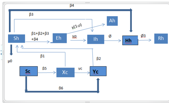
Figure 1. Flow chart for the transmission of MERS-CoV between camel and human population.
