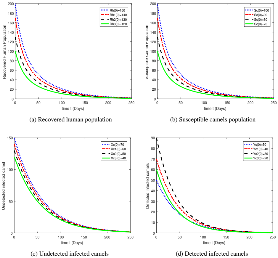
Figure 6. The plots demonstrate the time dynamics of different compartmental population recover, susceptible camels, undetected infected camels, detected infected camels when R_0 < 1 .
