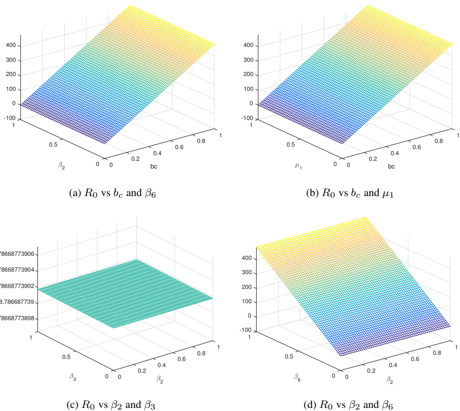
Figure 2. The graphs show the variation of different parameters and its effect on the basic reproductive number.
