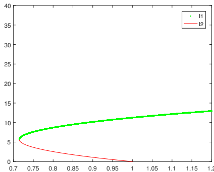
Figure 4. Bifurcation diagram of model (1) showing backward bifurcation.
