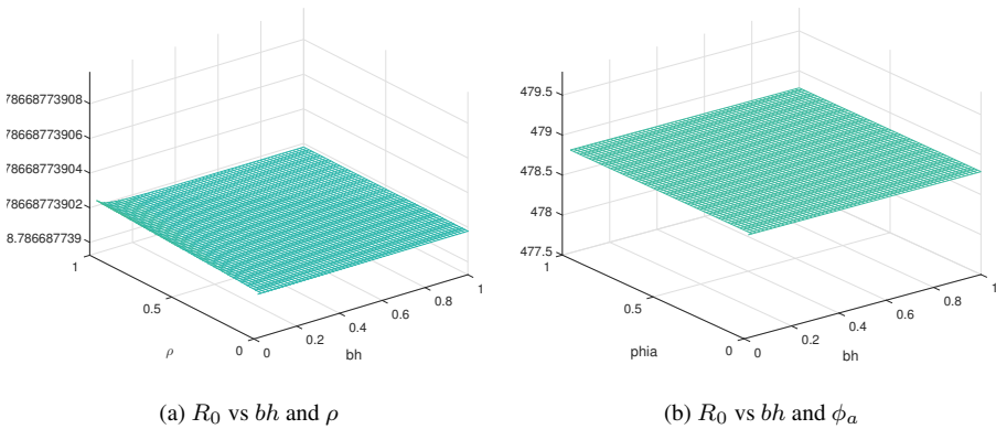
Figure 3. The graphs show the variation of different parameters and its effect on the basic reproductive number.
