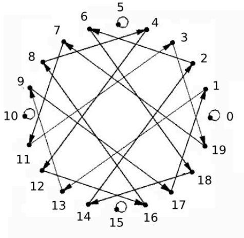
Figure 3: The orbit diagram for the critical points of F_{\lambda_0}(z) = z^{13} + \lambda_0/z^7 where \lambda_0 is the center of the principal Mandelbrot set \mathcal{M}_0 that intersects the positive real axis. The critical point on the positive real axis is a fixed point, and it is labeled with the number 0. The orbits of the remaining critical points are determined from the orbit of the fixed point using Symmetry Lemma 2.
