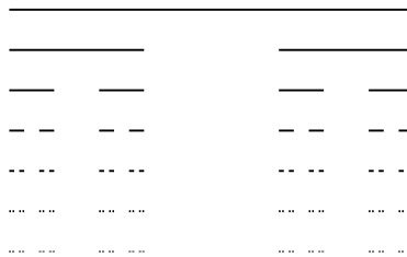
Figure 1: We present triadic Cantor set by iteration.
