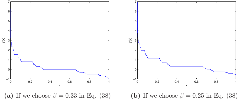
Figure 4: We draw the graph of Eq. (38).
