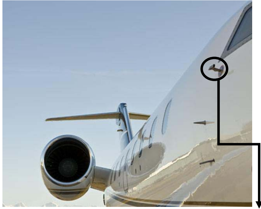
Figure 4 TAT Probe Installation on the A/C [8]
