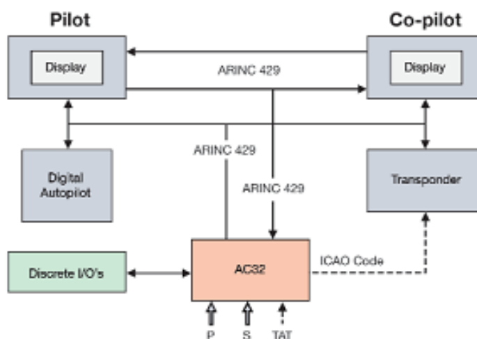
Figure 9 Typical Architecture of ADC Given by Manufacturer [16]
