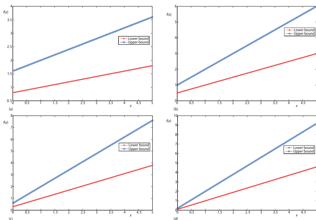
Figure 1. Interval solution with different fractional-order, \alpha , for eq. (8) over x \in [0, 5] ; (a) \alpha = 0.2 , (b) \alpha = 0.5 , (c) \alpha = 0.7 , and (d) \alpha = 0.9
