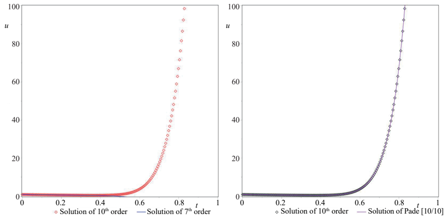
Figure 3. Comparison of the Adomian-Padé approximate solutions eq. (26) for the different steps 0 \leq t \leq 1 and 0 \leq u \leq 100 (for color image see journal web site)
