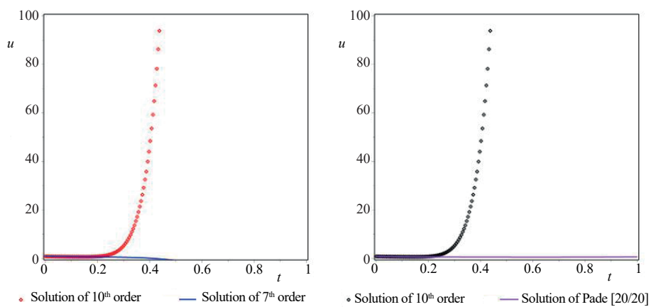
Figure 5. Comparison of the Adomian-Padé approximate solutions eq. (27) for the different steps 0 \leq t \leq 1 and 0 \leq u \leq 100 (for color image see journal web site)
