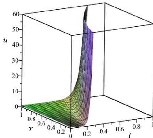
Figure 6. The decomposition solution for the 10 th - order series for 0 \leq x \leq 1 , 0 \leq t \leq 1 and 0 \leq u \leq 60 with eq. (2) (for color image see journal web site)
