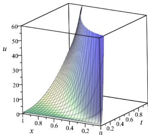
Figure 2: The decomposition solution for the 3 rd -order series for 0 \leq x \leq 1 , 0 \leq t \leq 1 and 0 \leq u \leq 60 with eq. (2) (for color image see journal web site)
