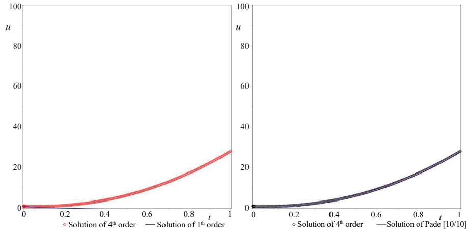
Figure 1. Comparison of the Adomian-Padé approximate solutions eq. (25) for the different steps and 0 \leq t \leq 1 and 0 \leq u \leq 100 (for color image see journal web site)
