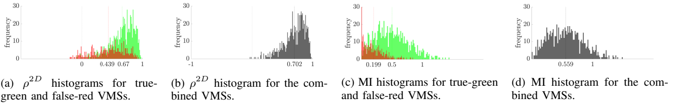
Fig. 6: Histograms of the average correlation ( \rho^{2D} ) and MI, between the VMS's corresponding to two equally sized groups of participants. The green histograms represent the correlation or MI for the true VMSs, while the red histograms correspond to those of the false VMSs.
