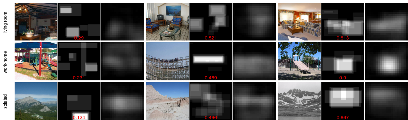
Fig. 12: Some examples of VMS reconstruction results when using transfer learning for the VGG-VD-19L structure at layer conv-5^2 , using l_1 -norm, for epoch 20. In each row, there are 3 images for 3 categories, each representing a poor, a moderate and a successful reconstruction result, from left to right, respectively. For each sample image, the images show the empirically collected VMS and that reconstructed using deep learning. The reconstruction accuracy is indicated by the correlation between the empirically collected and reconstructed VMS.
