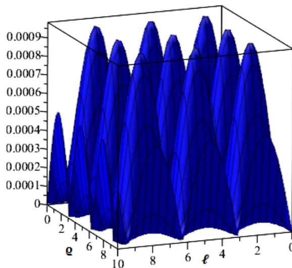
Figure 3. The solution graph of Example 2 (a) Exact solution and (b) ILTM solution at \rho = 1 .
