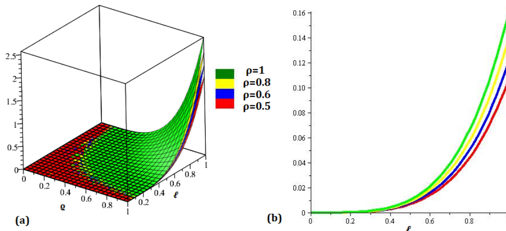
Figure 7. The (a) ISTM solution different fractional orders of Example 4 (b) \tau_1 = 0.5 .
