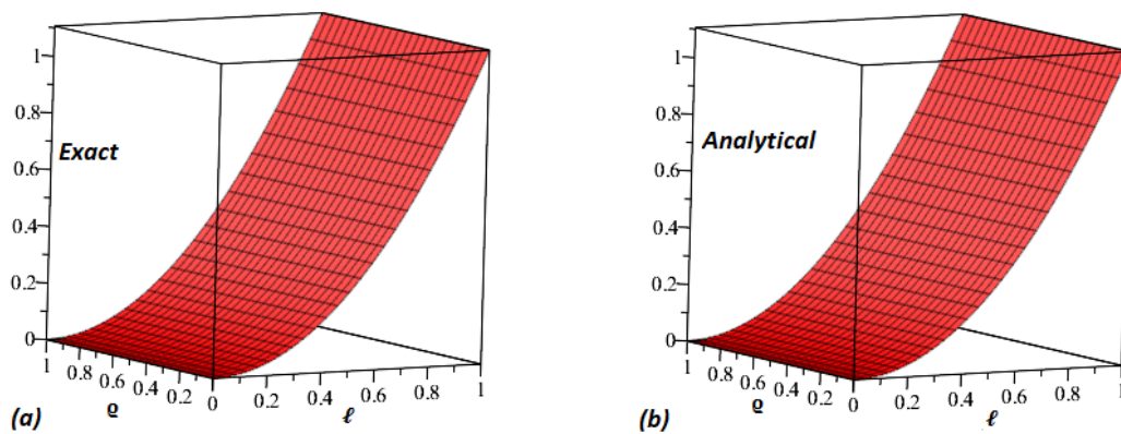
Figure 1. The solution graph of Example 1 (a) Exact solution and (b) ISTM solution at \rho = 1 .
