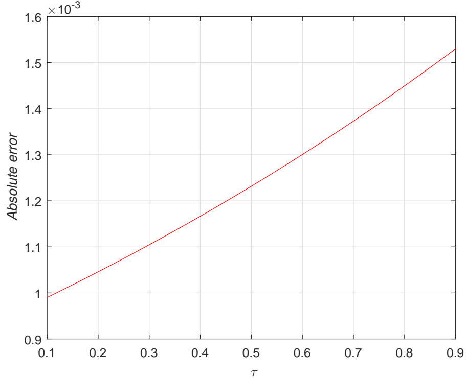
Figure 9. Absolute error between obtained solutions by BWM and ABM.
