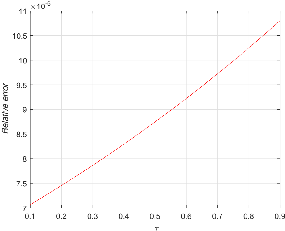
Figure 8. Relative error between obtained solutions by BWM and ABM.
