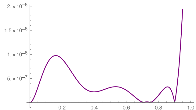
Fig. 2 Plots of absolute error for N = 7 .
