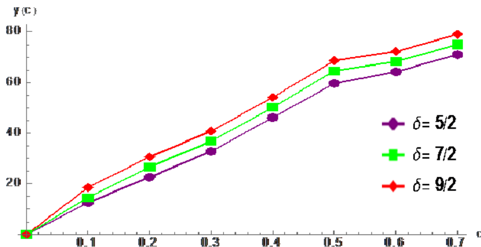
Figure 2. Solution of Eq (5.2).
