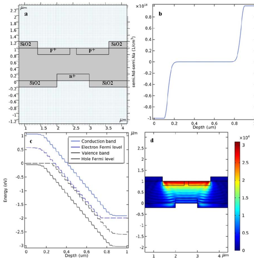
Fig. 1 (a) Device Structure Without NP; (b) Doping Profile Graph 1/cm 3 ; (c) Energy Level Diagram; (d) 2-D Electric Field Graph (V/m) at \lambda = 870 nm
