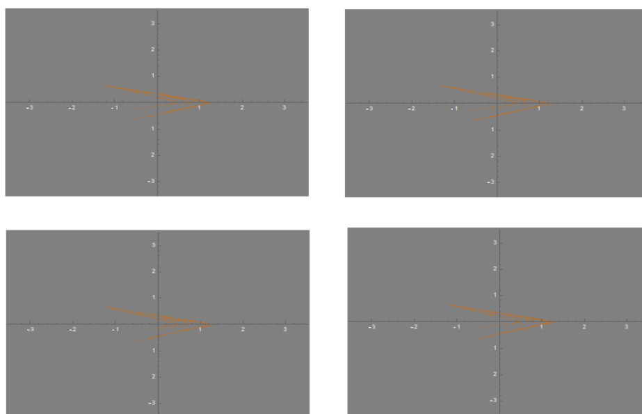
Figure 2. The behavior of the discrete VFLM, when (\alpha, \beta) = (1.7, 0.5) . From the left \varphi(v) = \sin\left(\frac{1}{1+v}\right) , \varphi(v) = \sin\left(\frac{1}{0.1+v}\right) , \varphi(v) = \sin\left(\frac{1}{0.01+v}\right) and \varphi(v) = \sin\left(\frac{1}{0.001+v}\right) , v \in \mathbb{N} . The iteration is running from 1 to 1000.
